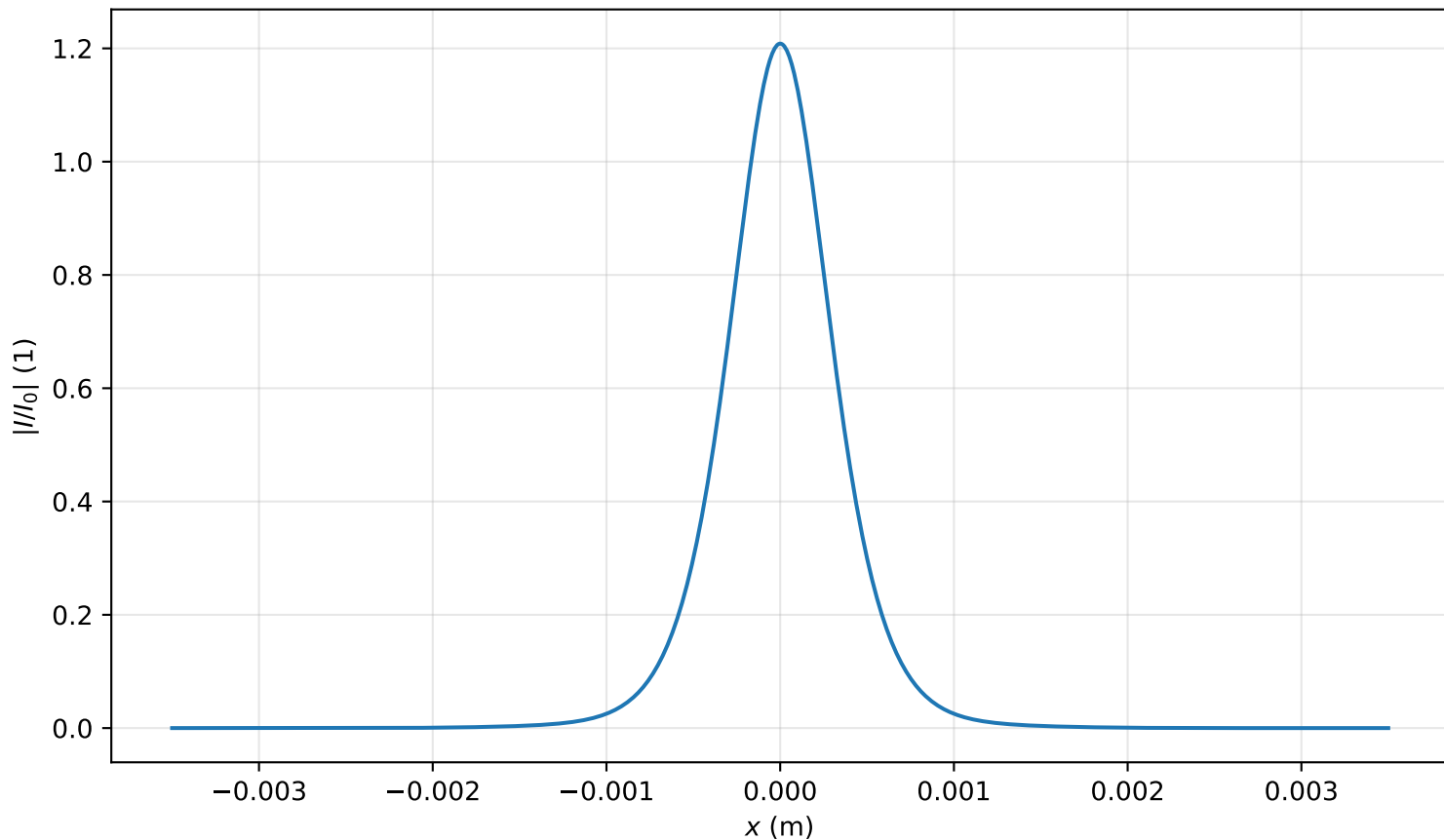
Intensity profile I(x, y = 0, z = 2.548m)/I_0 , P_{in}=0.8P_{cr} , artificial time
